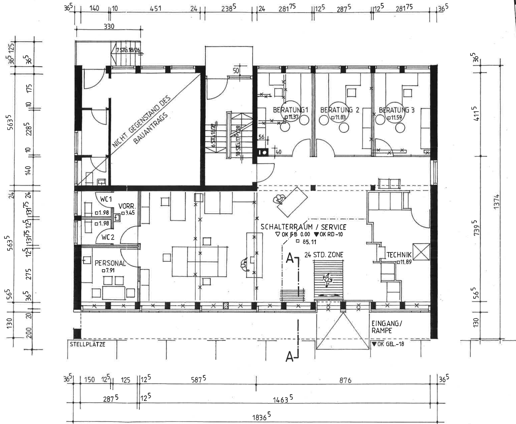
GRUNDRISS ERDGESCHOSS (BANKFILIALE)
